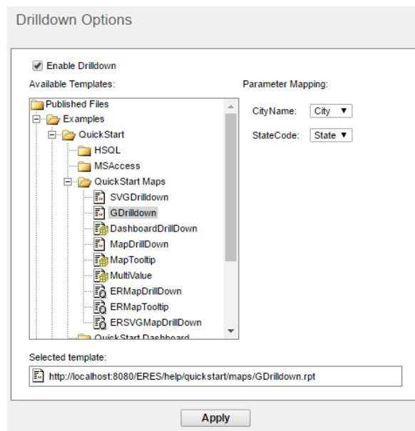
Drilldown Options
