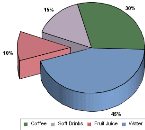
Pie Chart
