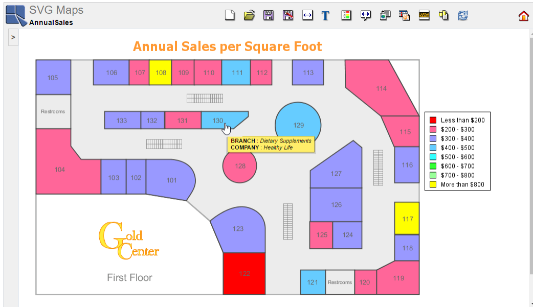
Finished Map
