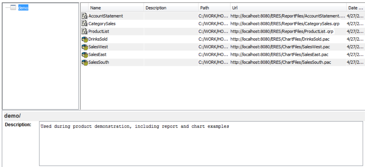
John's Organizer
