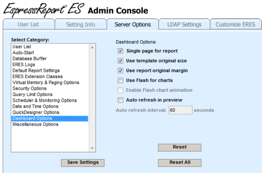
Dashboard Options
