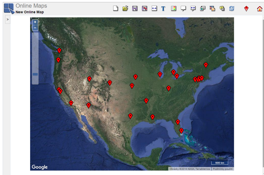
Google Satellite
