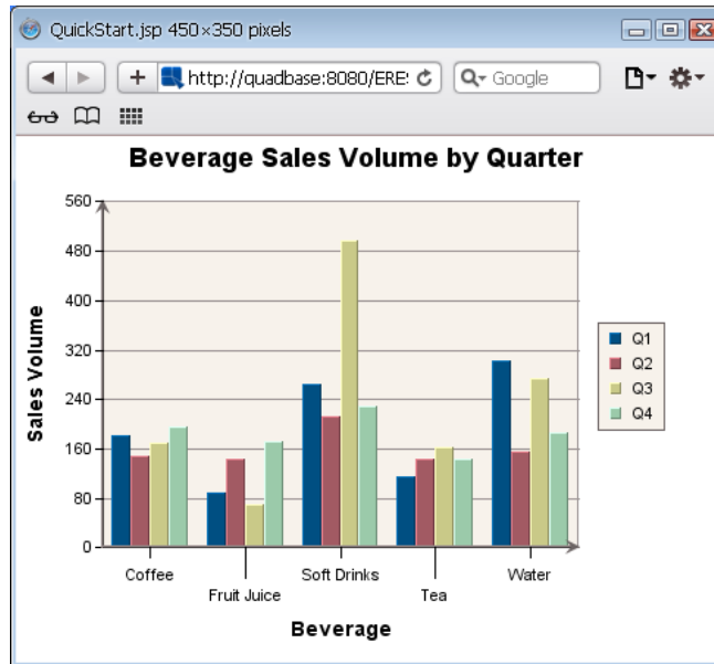
Chart Generated
