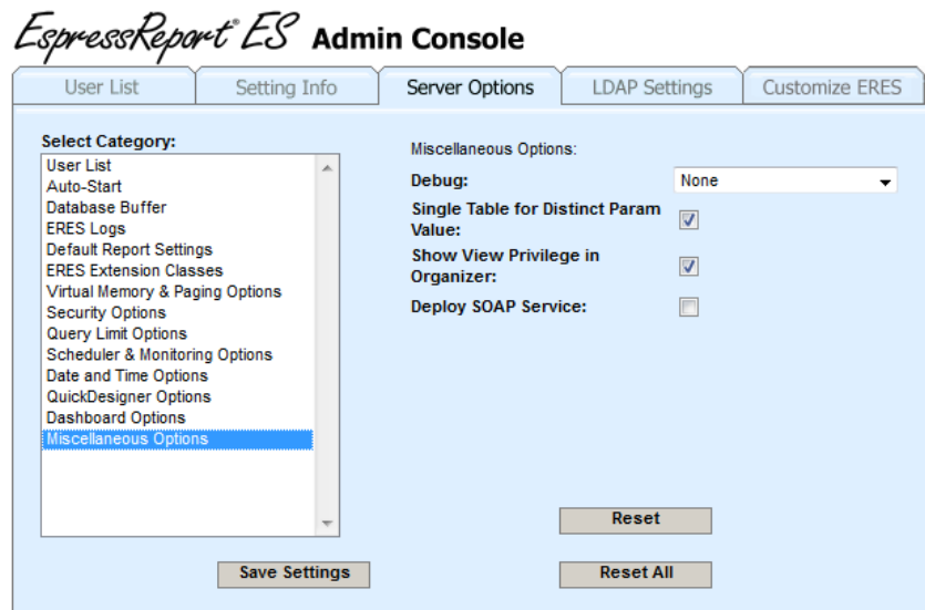
Miscellaneous Options
