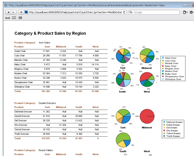
Report Generated
