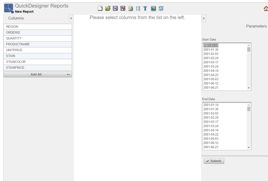
QuickDesigner Reports
