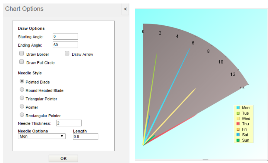
Circular Sector
