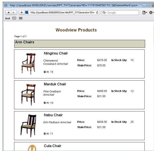
Report Generated
