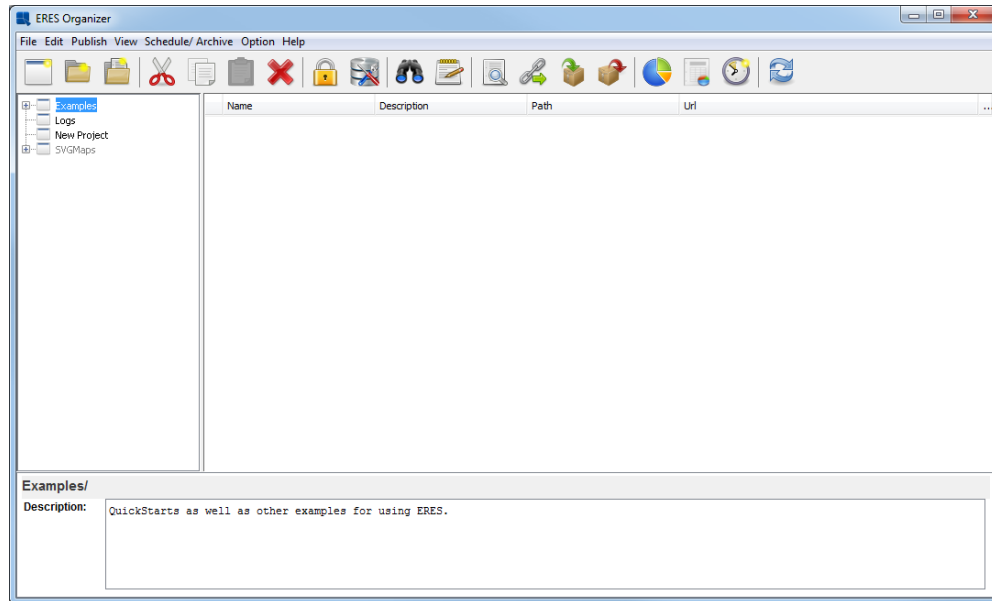
Organizer Interface
