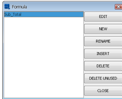
Formula List
