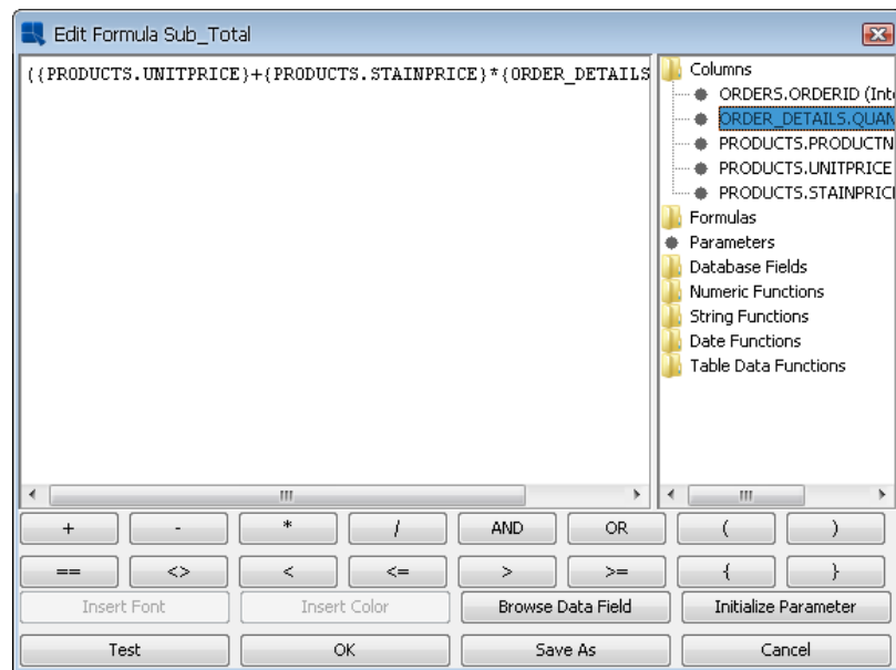
Formula Editor
