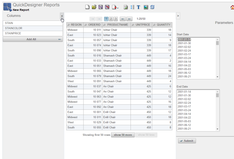
Collapse Sidebars
