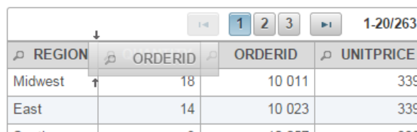
Column Order
