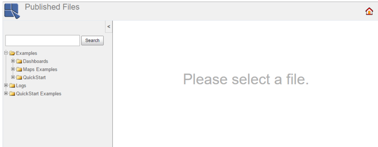
Menu Page
