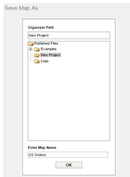
Save Dialog
