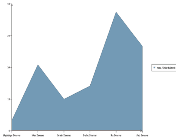
Generated chart
