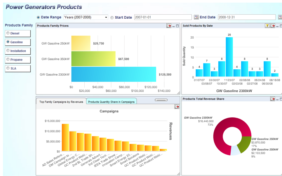
Dashboard
