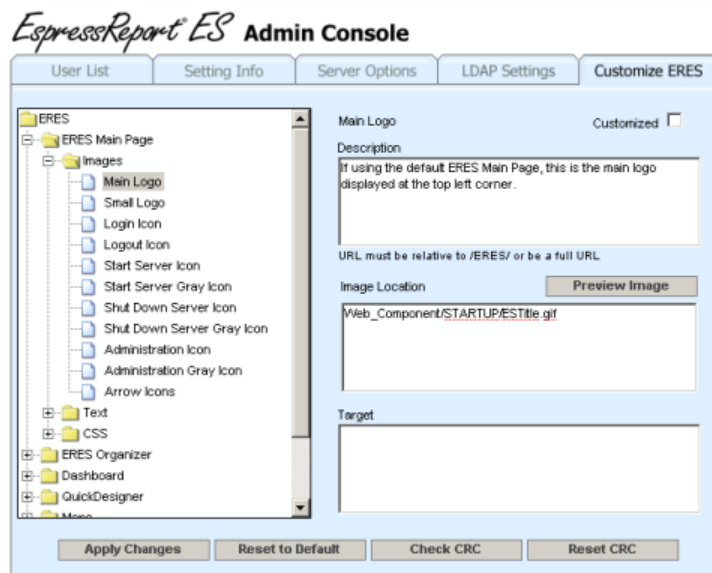
Preview Image
