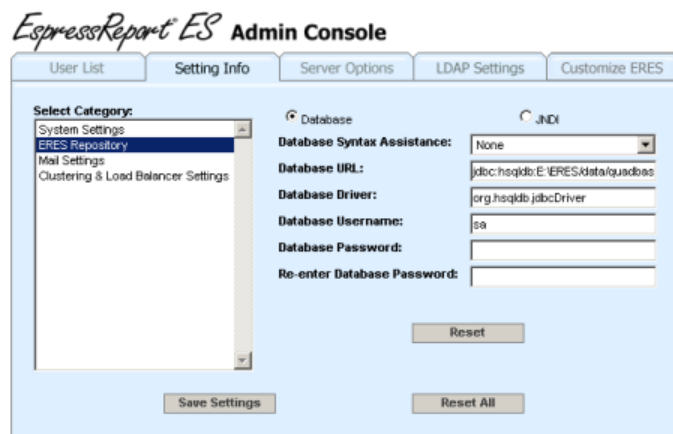
Database Repository
