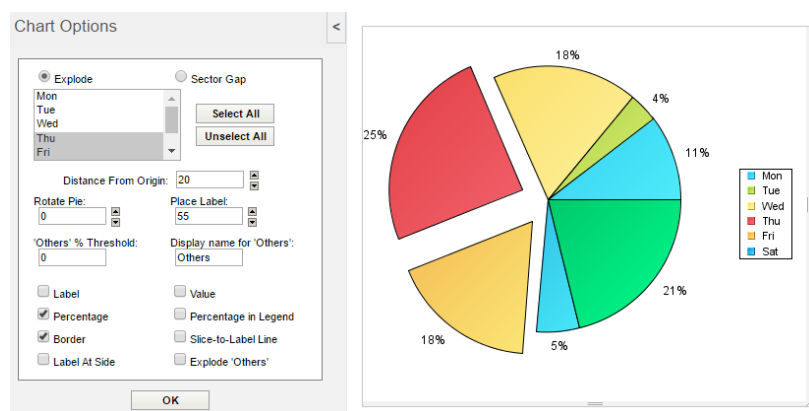
Exploded Slices
