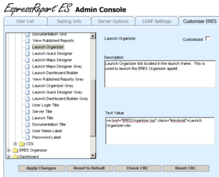
Customizing Text
