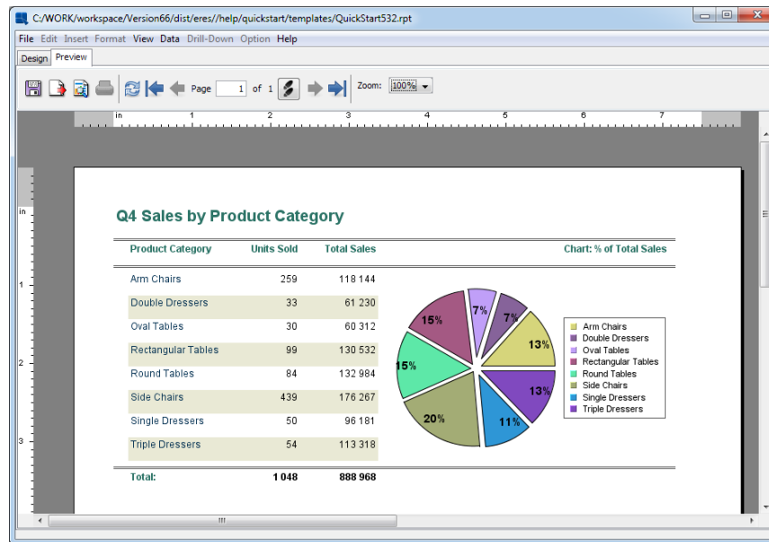
Preview Window
