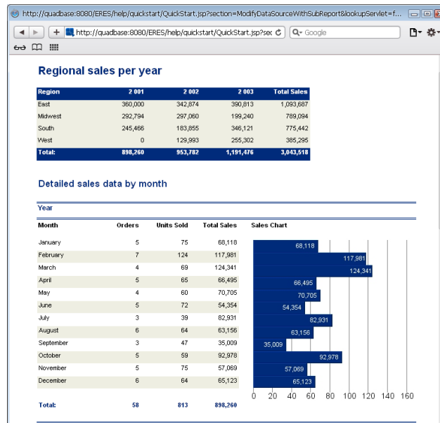
Report Generated
