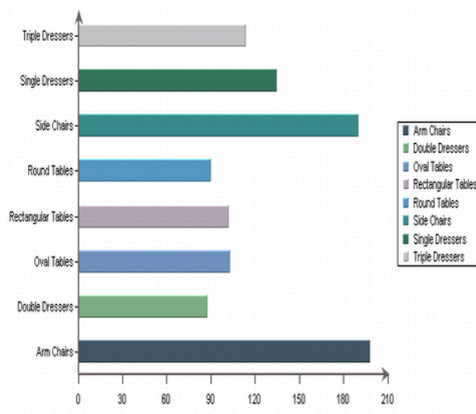
Generated chart
