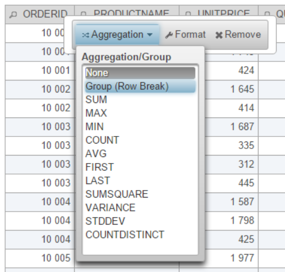
Aggregation/Group Setting
