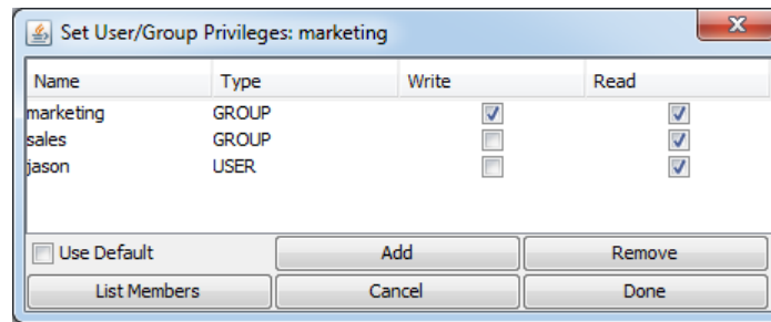
Group/User Permissions
