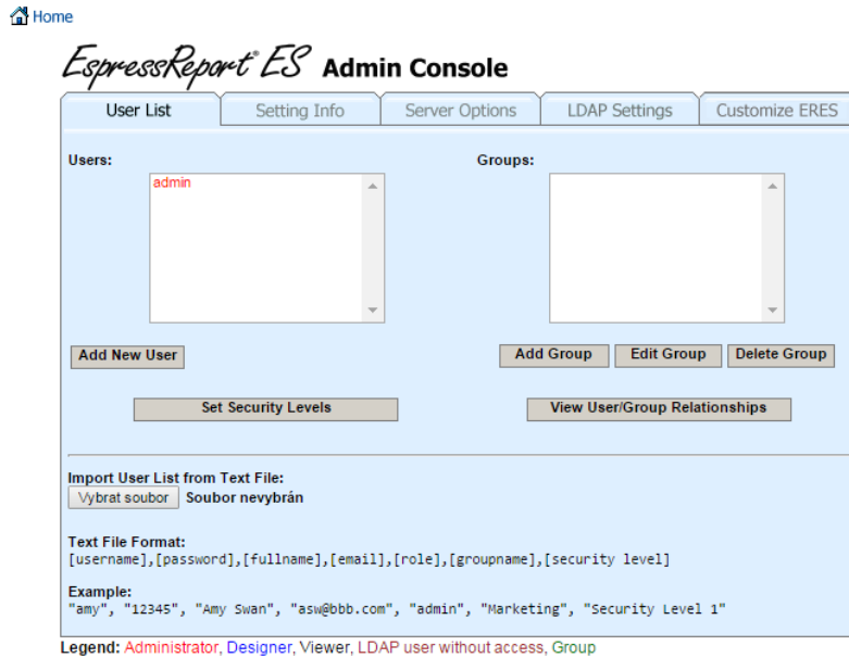
Admin Console
