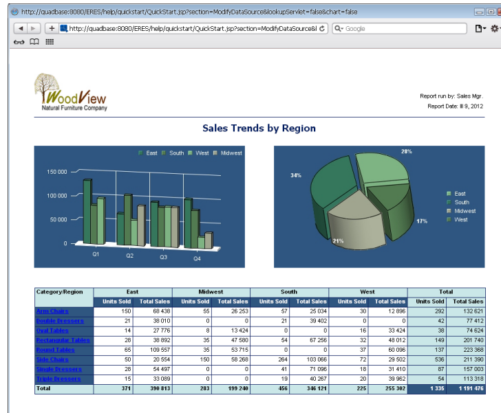
Report Generated
