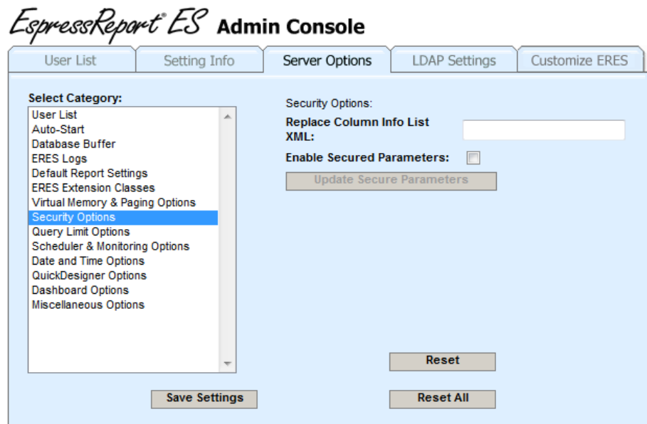
Security Options
