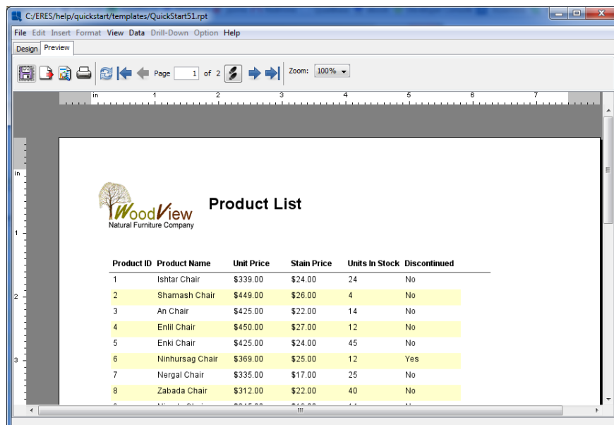
Finished Report
