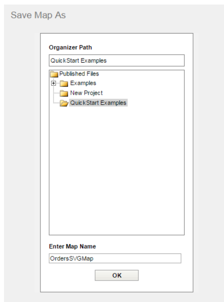
Saving Map
