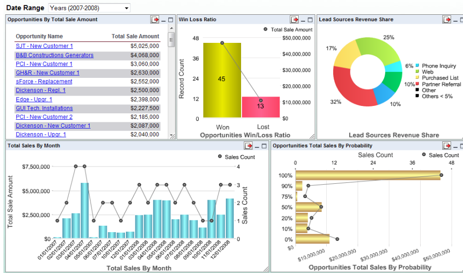
Products Dashboard
