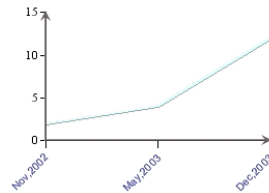
Example Results
