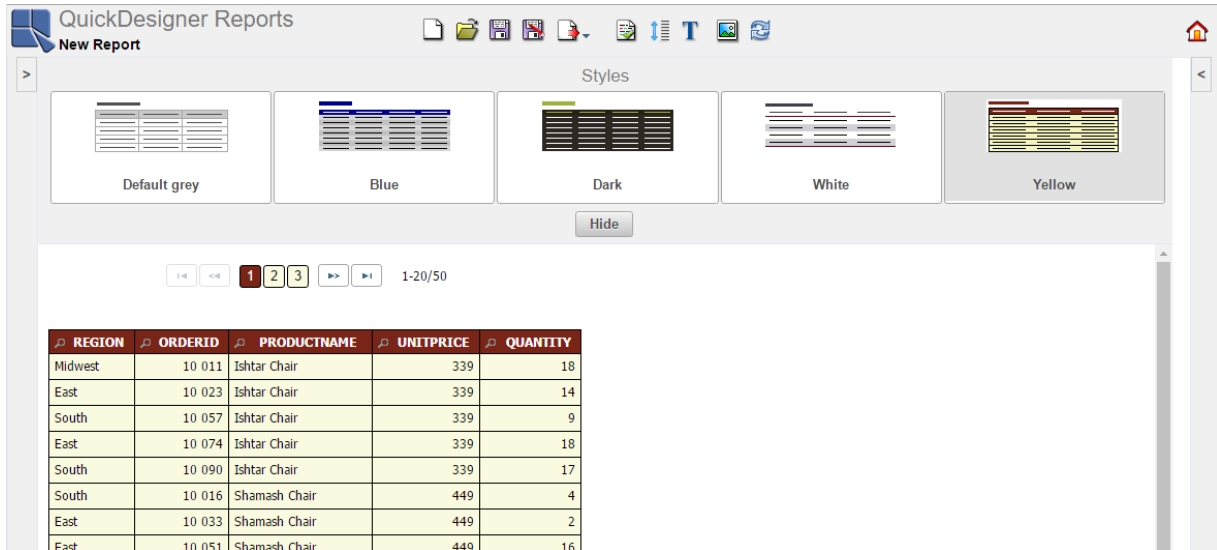
Styles Dialog
