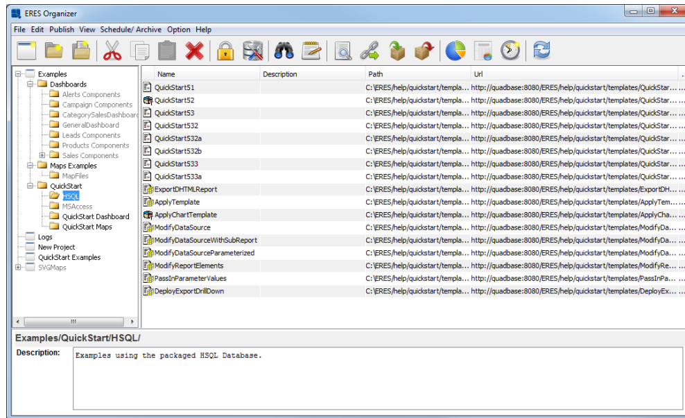
Organizer Interface
