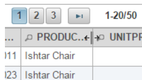
Column Width
