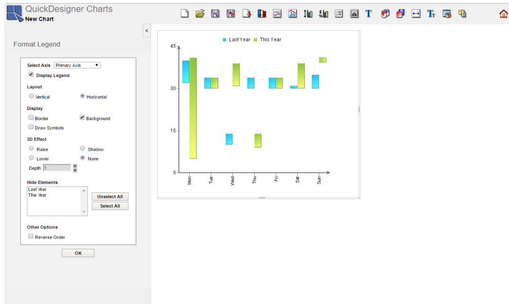
Finished Chart
