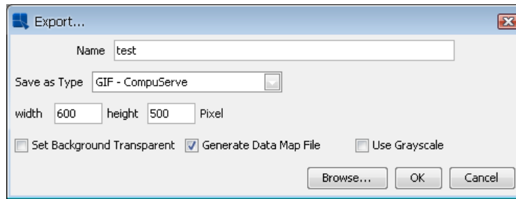
Export Dialog
