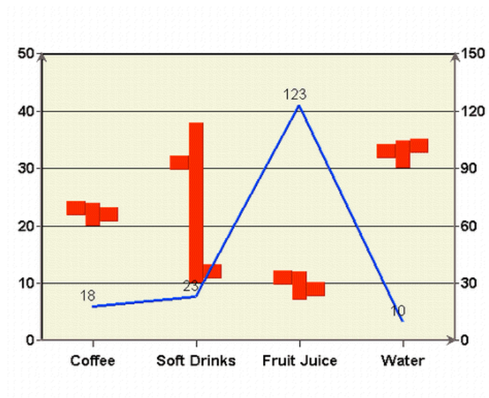
Streaming Chart
