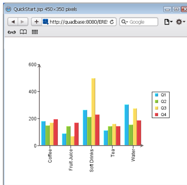
Chart Generated
